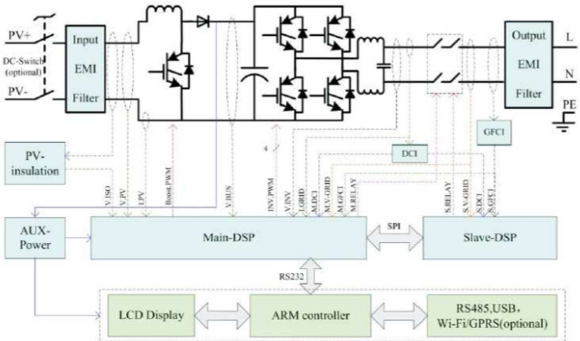
PGU Block Diagram:
